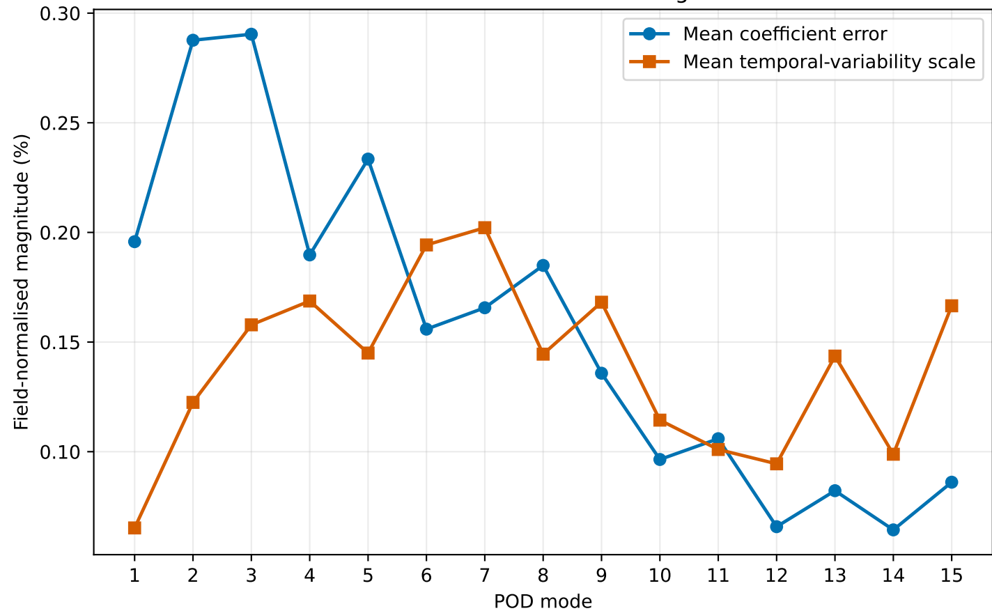
Rank-15 external coefficient diagnostics
