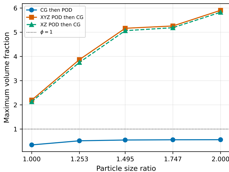
Rank-100 maximum volume fraction
