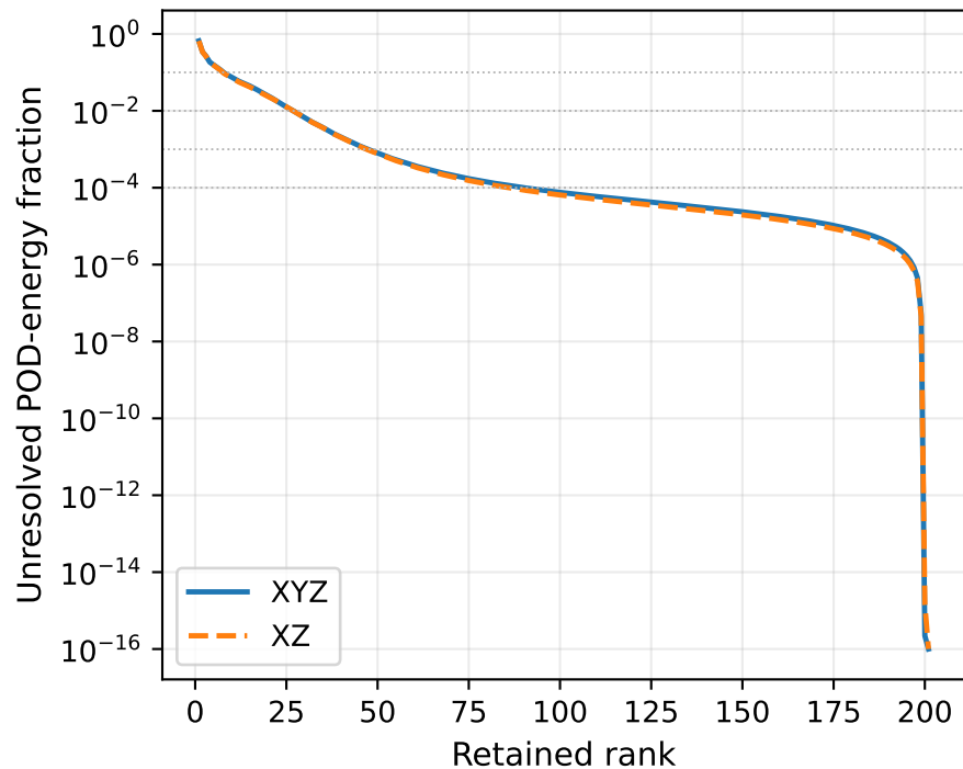
Truncation tail
