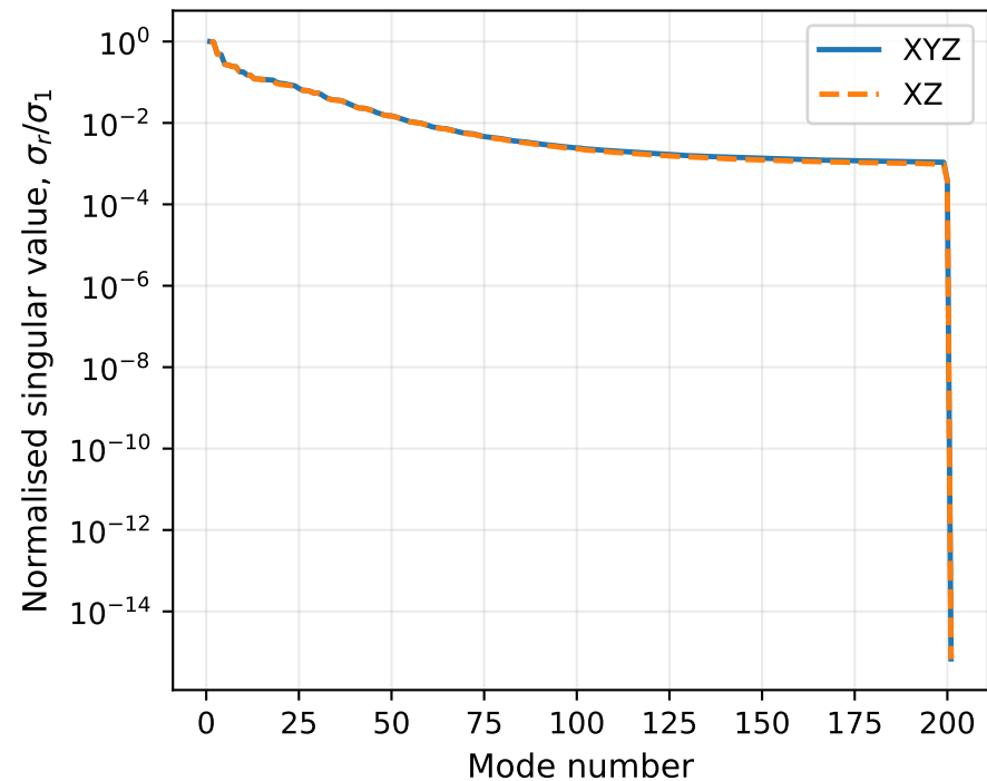
Singular-value decay
