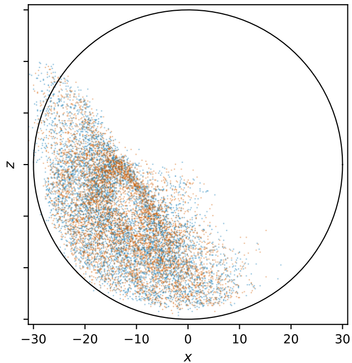
Rank 100 labelled RMSE = 10.11, NN RMSE = 1.04
