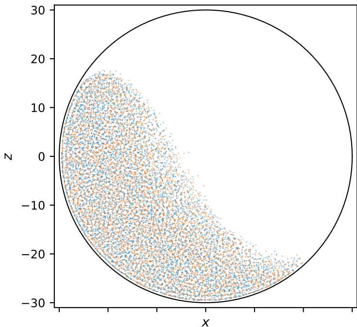
Rank 27 labelled RMSE = 10.23, NN RMSE = 1.03
