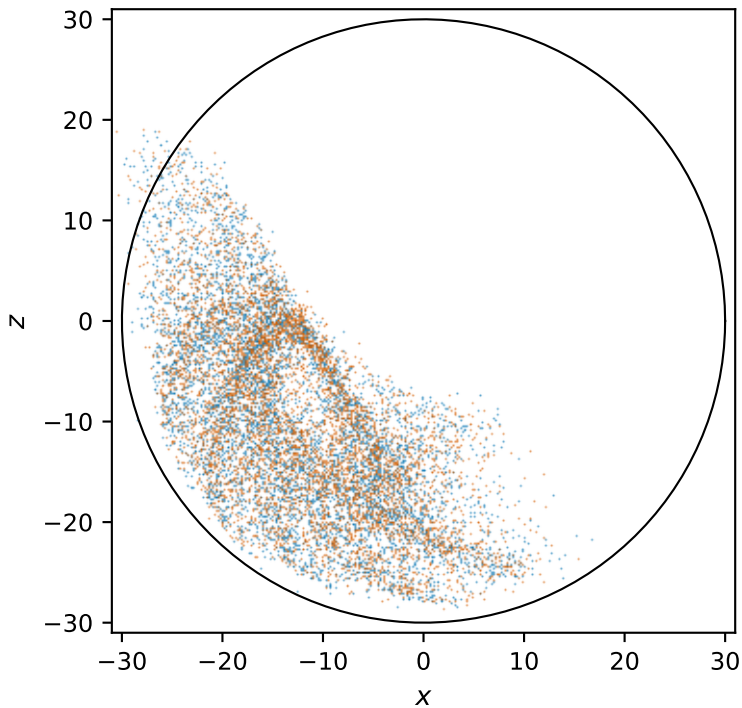
Rank 27 labelled RMSE = 10.23, NN RMSE = 1.03
