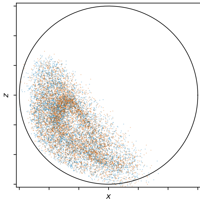
Rank 100 labelled RMSE = 10.11, NN RMSE = 1.04
