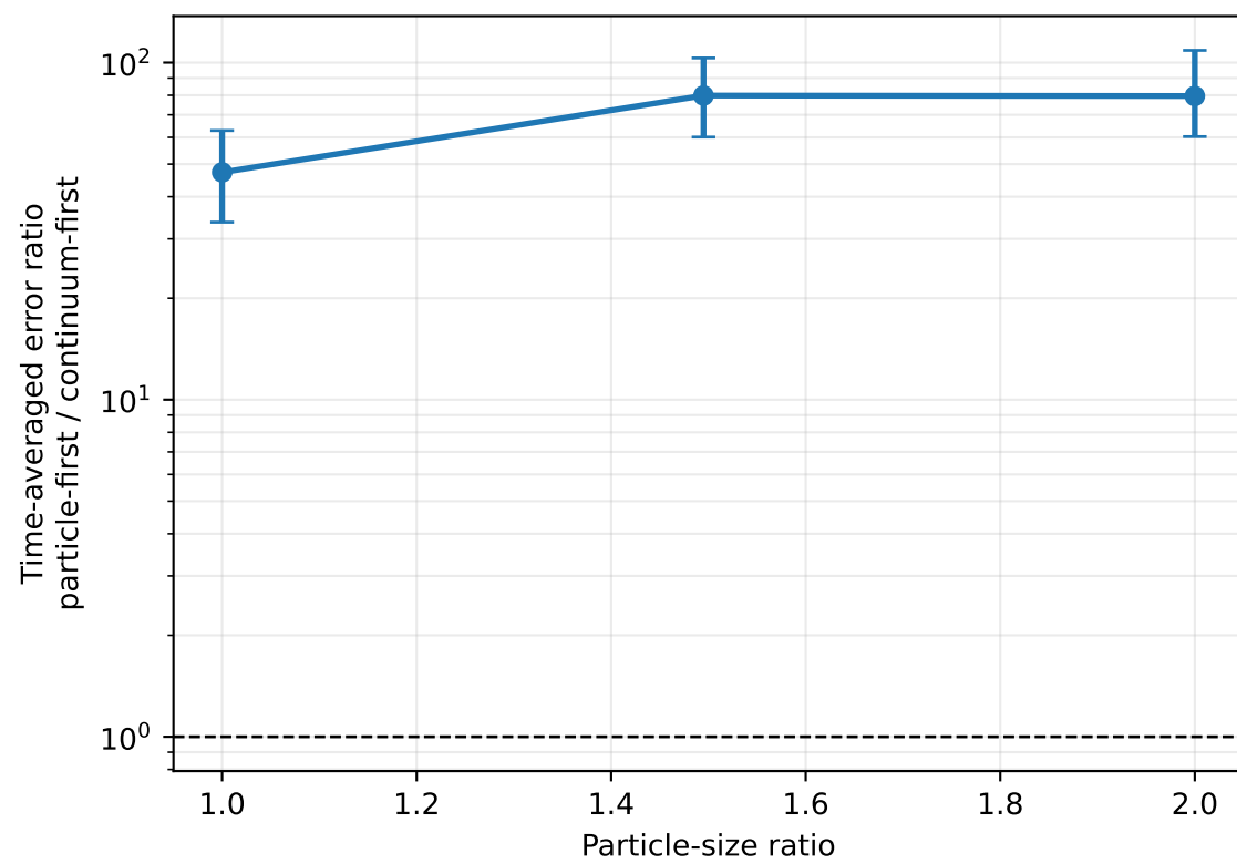
Rank 100
