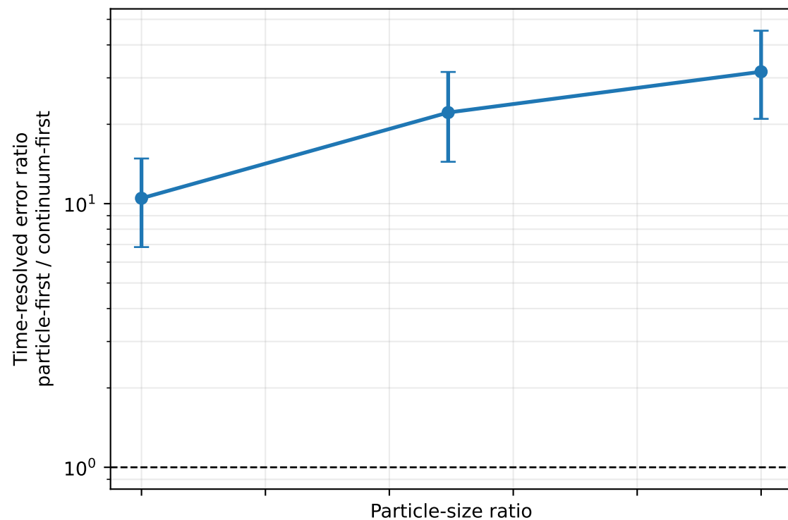
Rank 100
