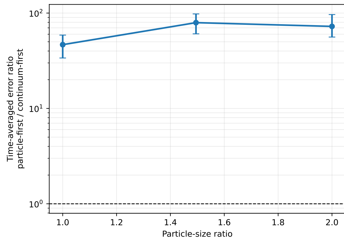
Rank 27
