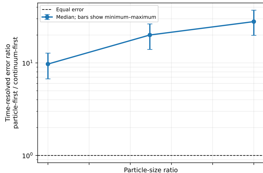
Rank 27
