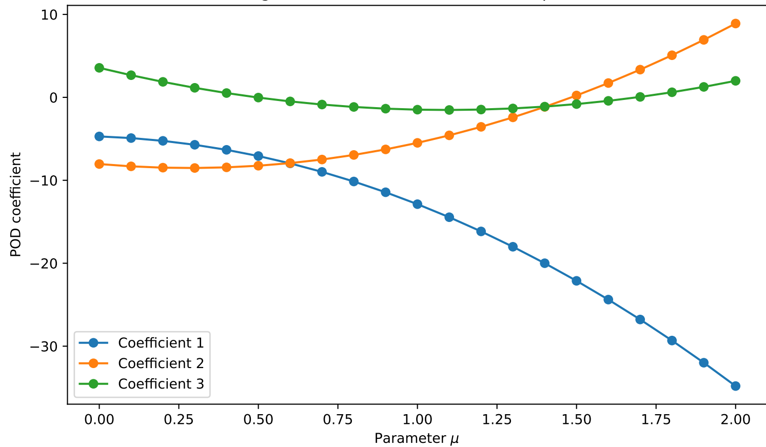
Training POD coefficients as functions of parameter
