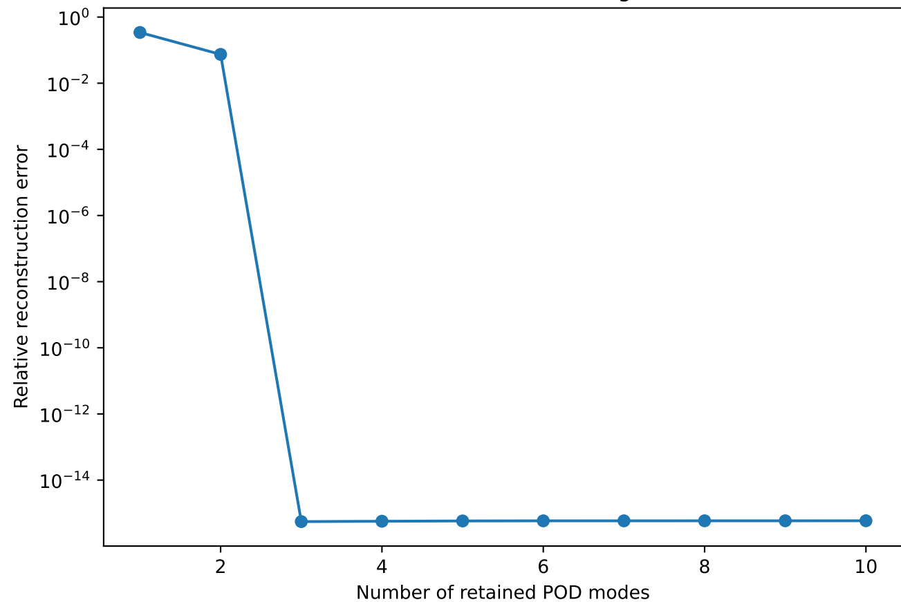
POD reconstruction convergence
