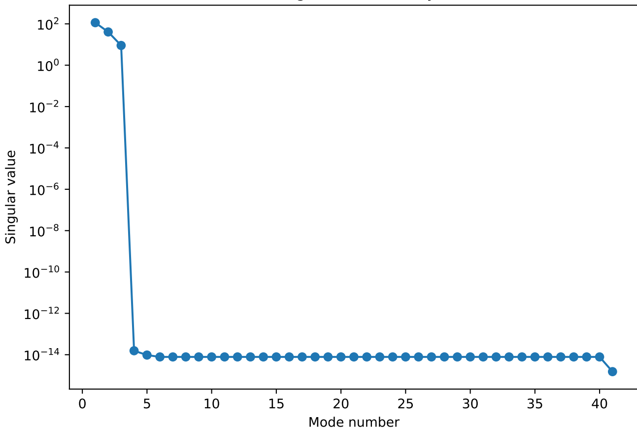
Singular-value decay
