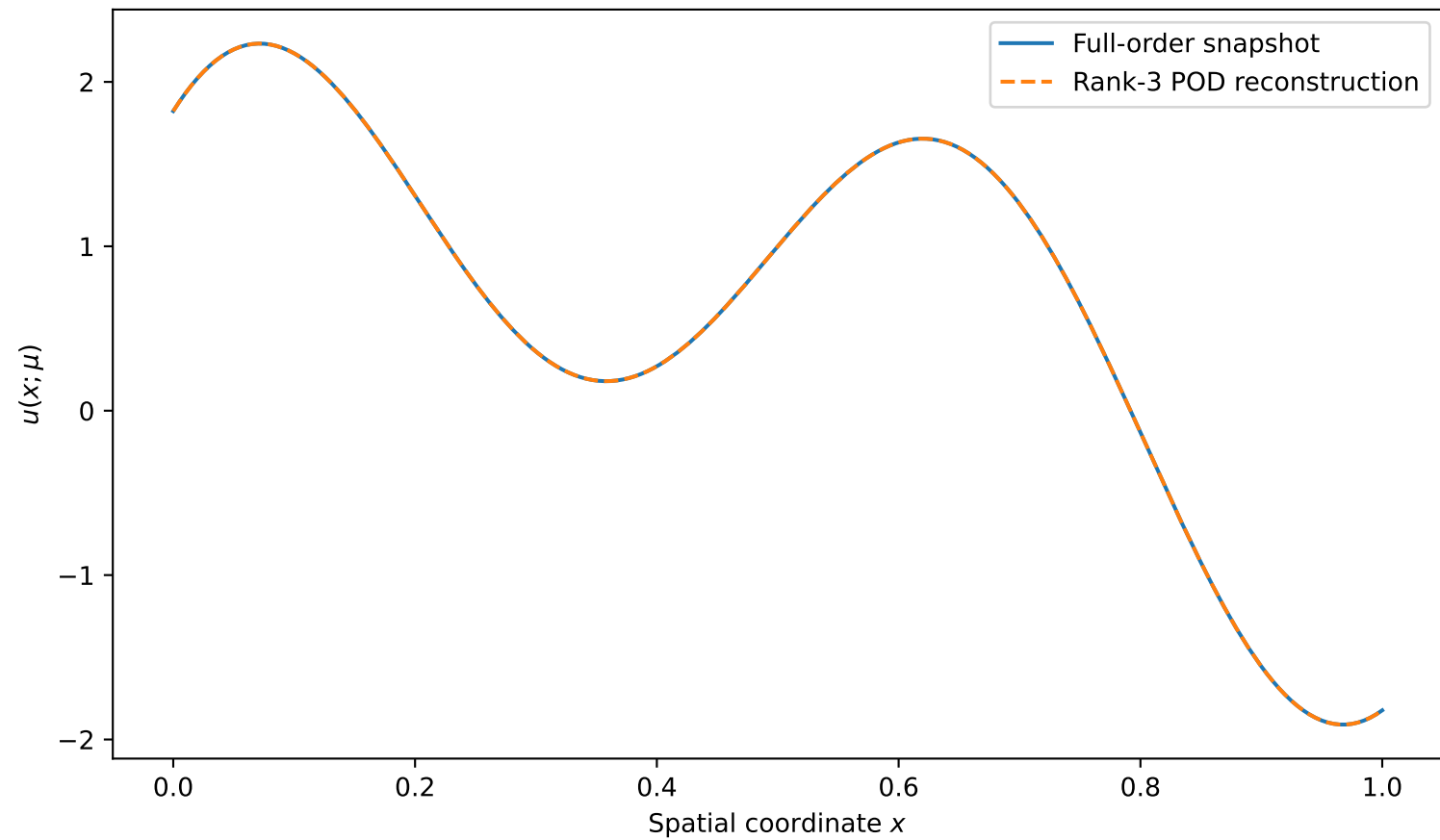
Reconstruction at \mu = 1.35
