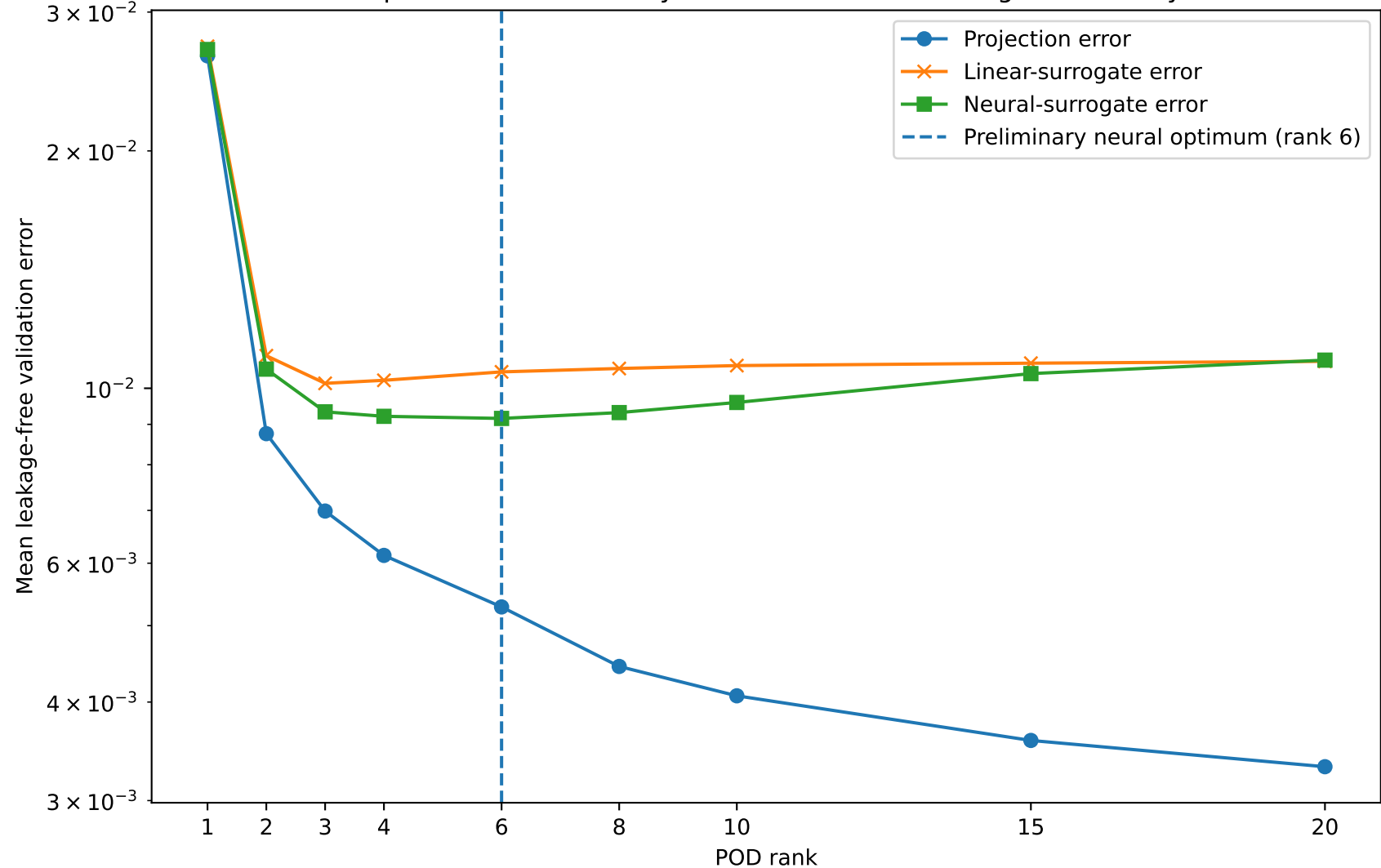
Representation accuracy versus end-to-end surrogate accuracy
