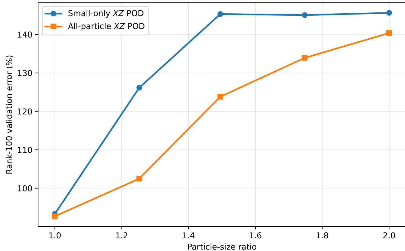
Observable-matched versus all-particle XZ POD
