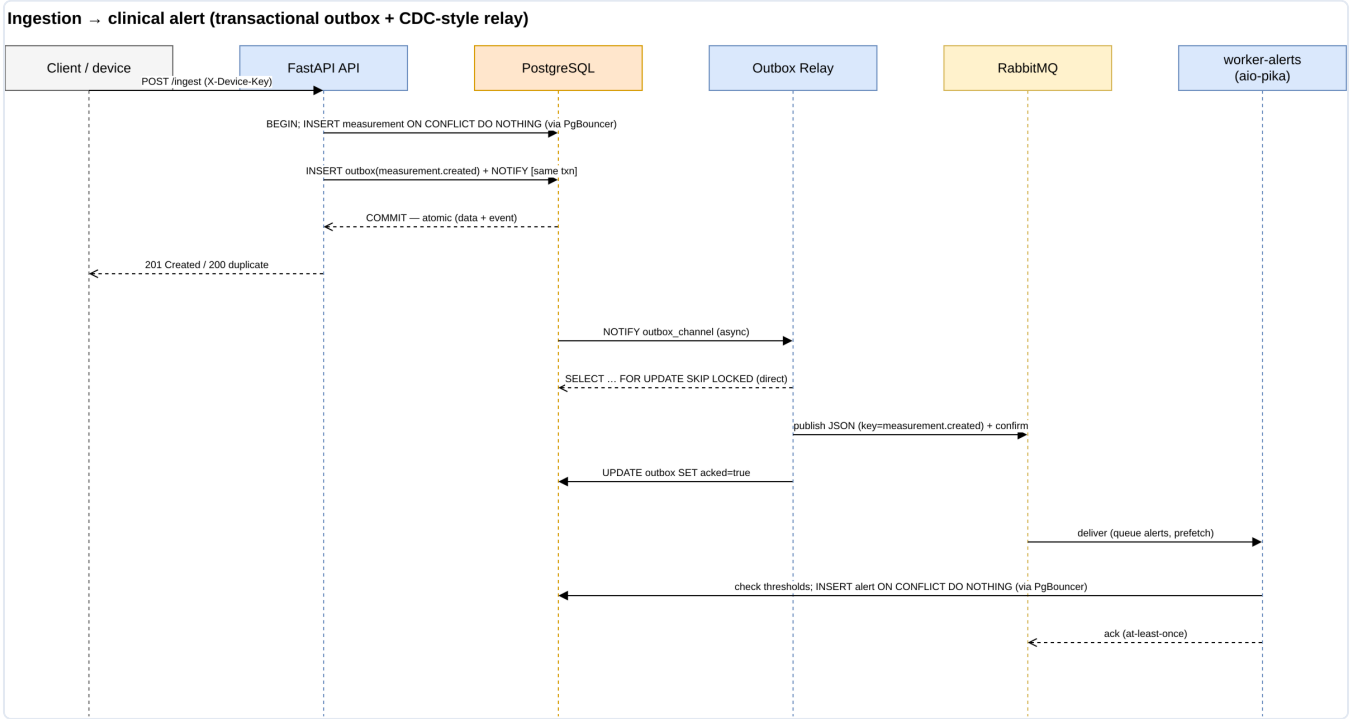
Figure 3 — Ingest → clinical alert. The red boundary in the narrative is the atomic write (measurement + outbox row + NOTIFY); everything after the relay is at-least-once with an exactly-once effect.
