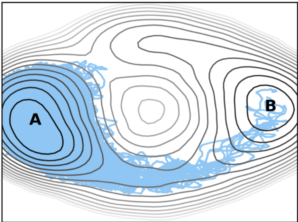
Metadynamics transition paths
