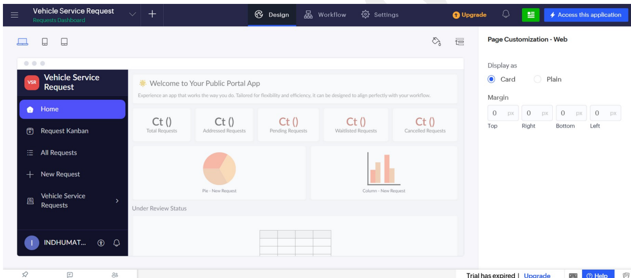
Figure 9.5: Zoho Creator Application Editor – Design Area
