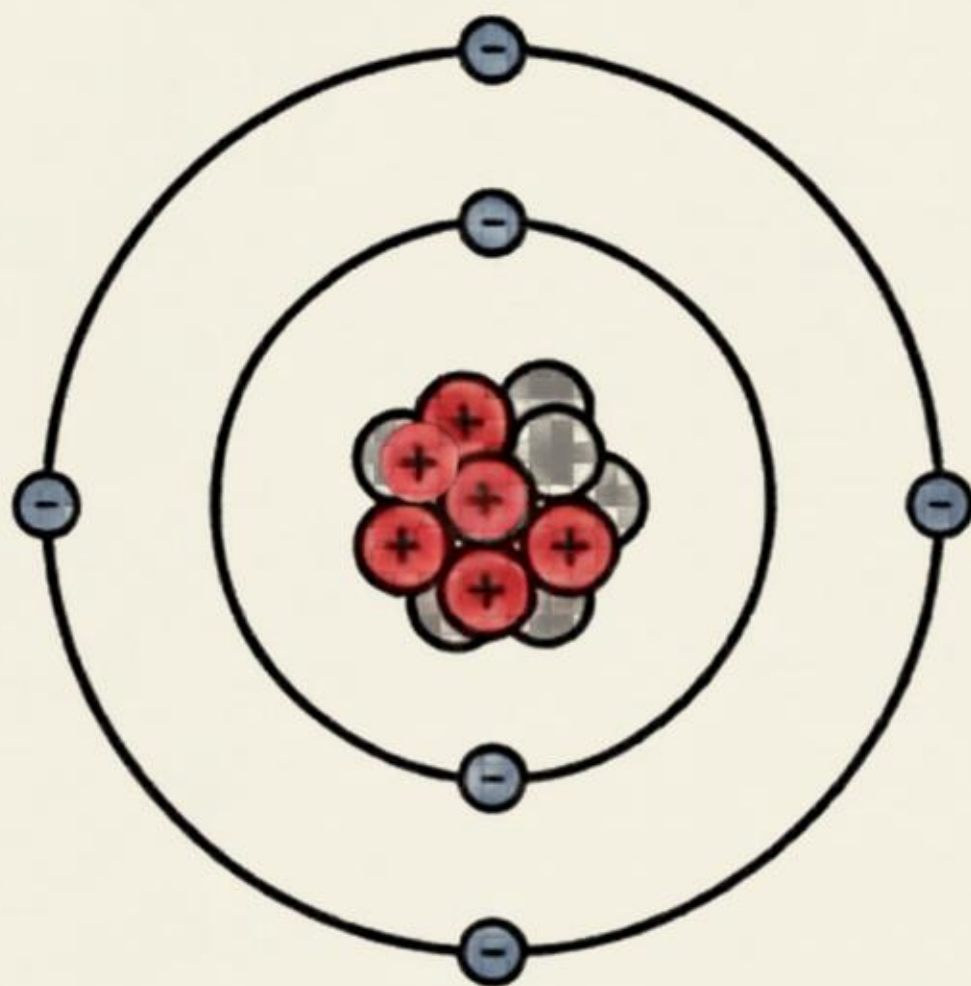
Carbon (6p, 6n)
