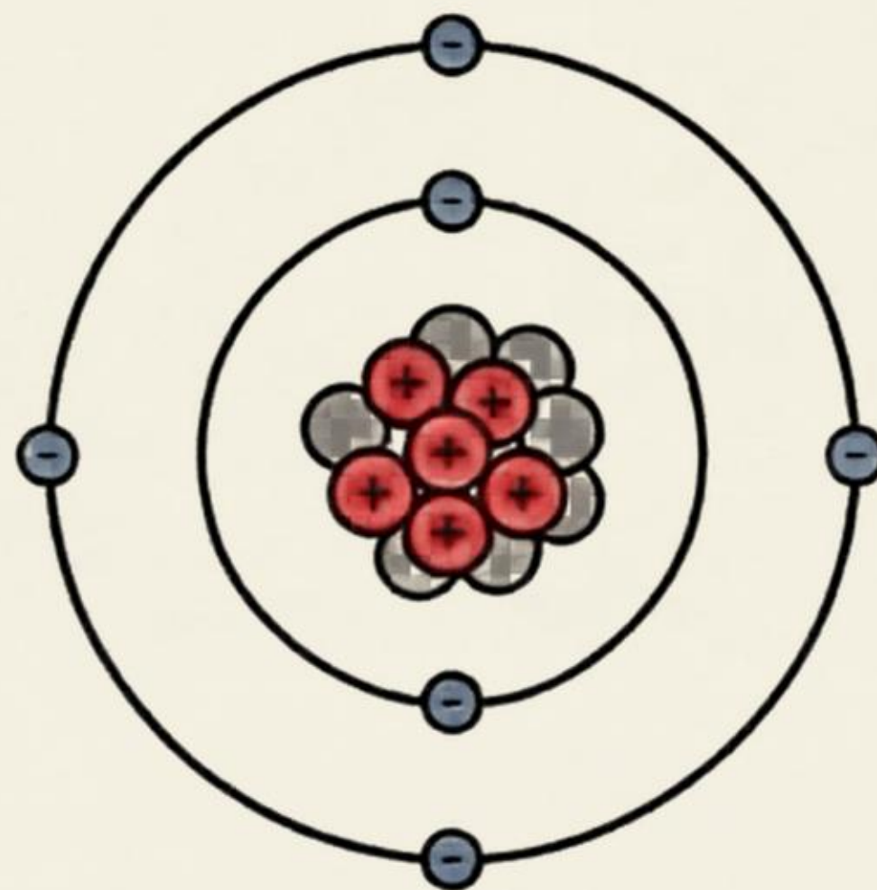
Carbon (6p, 7n)
