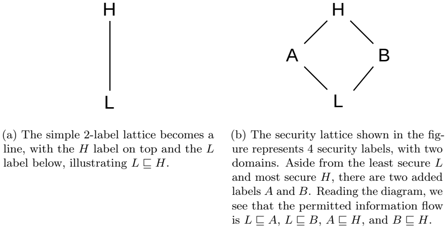
Figure 2.3: Hasse diagrams for our previously presented 2-label lattice and a new 4-label lattice. The orientation of the diagram matters, in that the higher up in the diagram a label appears, the higher its security position in the lattice.
