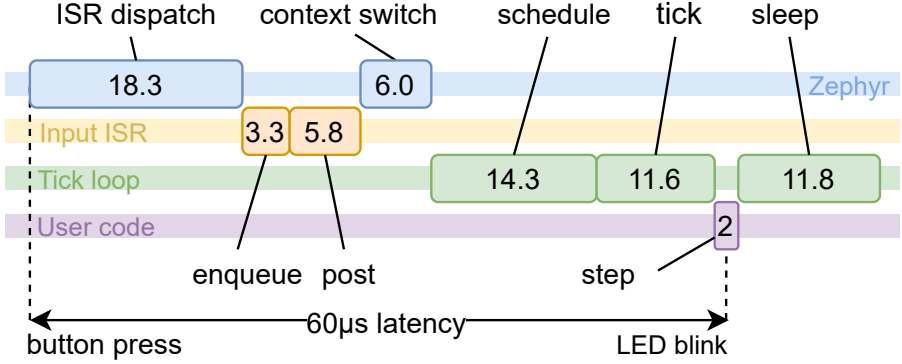
Fig. 16. Timeline in \mu\text{s} of a single button press of “button-to-blink” (Figure 15), reconstructed from GPIO profiling.
