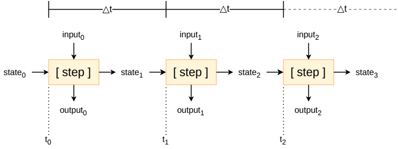
Figure 2.2: The figure illustrates how the step function is invoked periodically with \Delta t time elapsing between invocations. Within an instant time does not advance, so throughout the first invocation of step the time is always t_0 . As long as the invocation of step finishes before the next time of invocation, the observed behaviour of the system will be faithful to the synchronous model, with computation appearing instantaneous.
