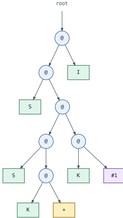
Figure 1.1: The combinator graph the MicroHs runtime builds in memory from the serialised representation of suc . Application nodes are drawn as circles; combinators and primitive operations are drawn as leaves.
