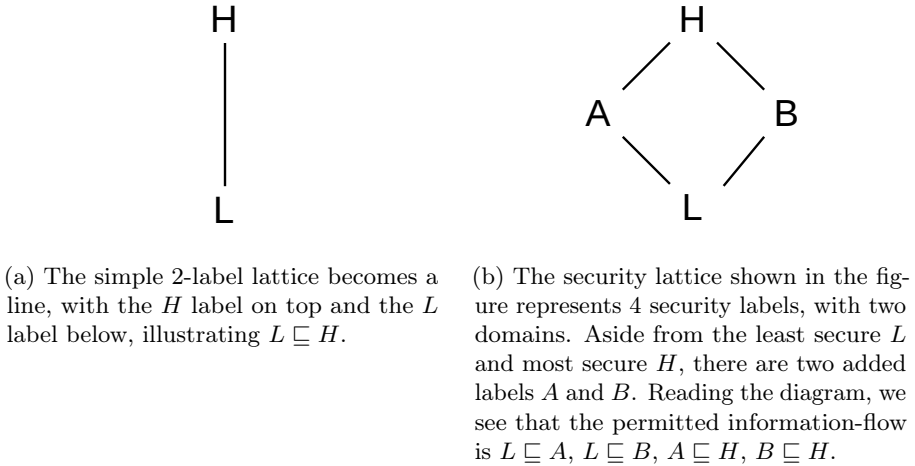
Figure 1.3: Hasse diagrams for our previously presented 2-label lattice, and a new 4-label lattice. The orientation of the diagram matters, in that the higher up in the diagram a label appears, the higher its security position in the lattice.
