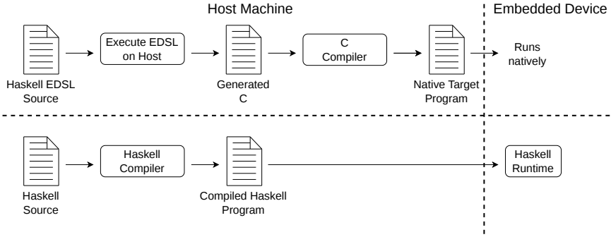
Figure 1.11: Two approaches to using Haskell for embedded programming. In the code-generation approach (top), a Haskell EDSL is executed on the host to produce C, which is compiled into a native target program. In the on-device execution approach (bottom), an ordinary Haskell program is compiled into an implementation-specific representation that is evaluated by a Haskell runtime on the embedded device.
