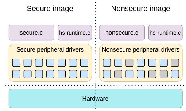
Figure 5: The Secure and Non-secure firmware images, each built from its generated MicroHasTEE C file and the MicroHas runtime on top of that domain's peripheral drivers, running on the shared hardware. The CMSE import library that the Secure build produces is omitted, as it is an artifact used by the linker, and is not present at runtime.
