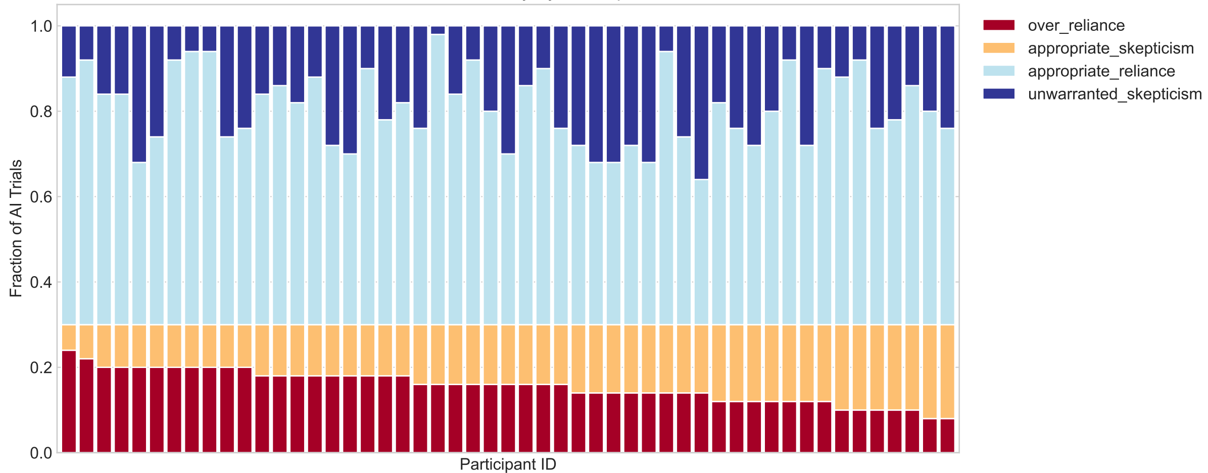
Reliance Taxonomy by Participant
