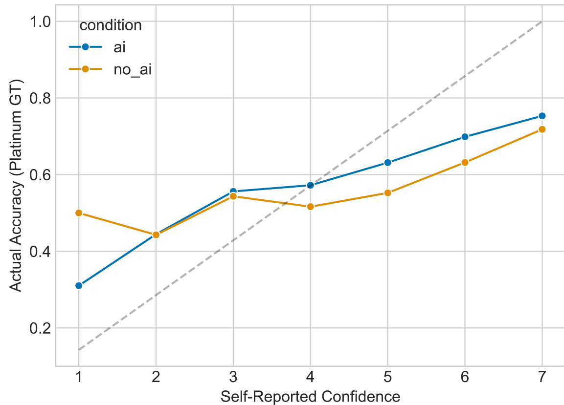
Confidence Calibration
