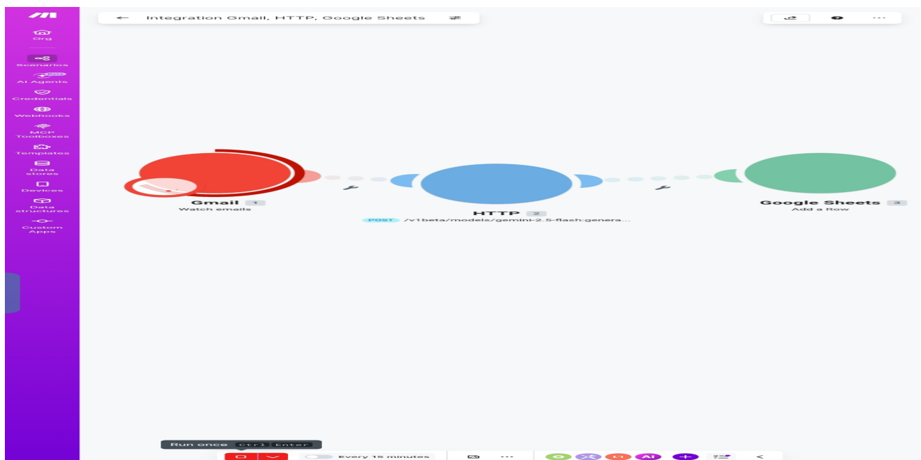
Screenshot 2: Make.com workflow diagram — Gmail (Watch emails) → HTTP (Gemini AI) → Google Sheets (Add a Row)
