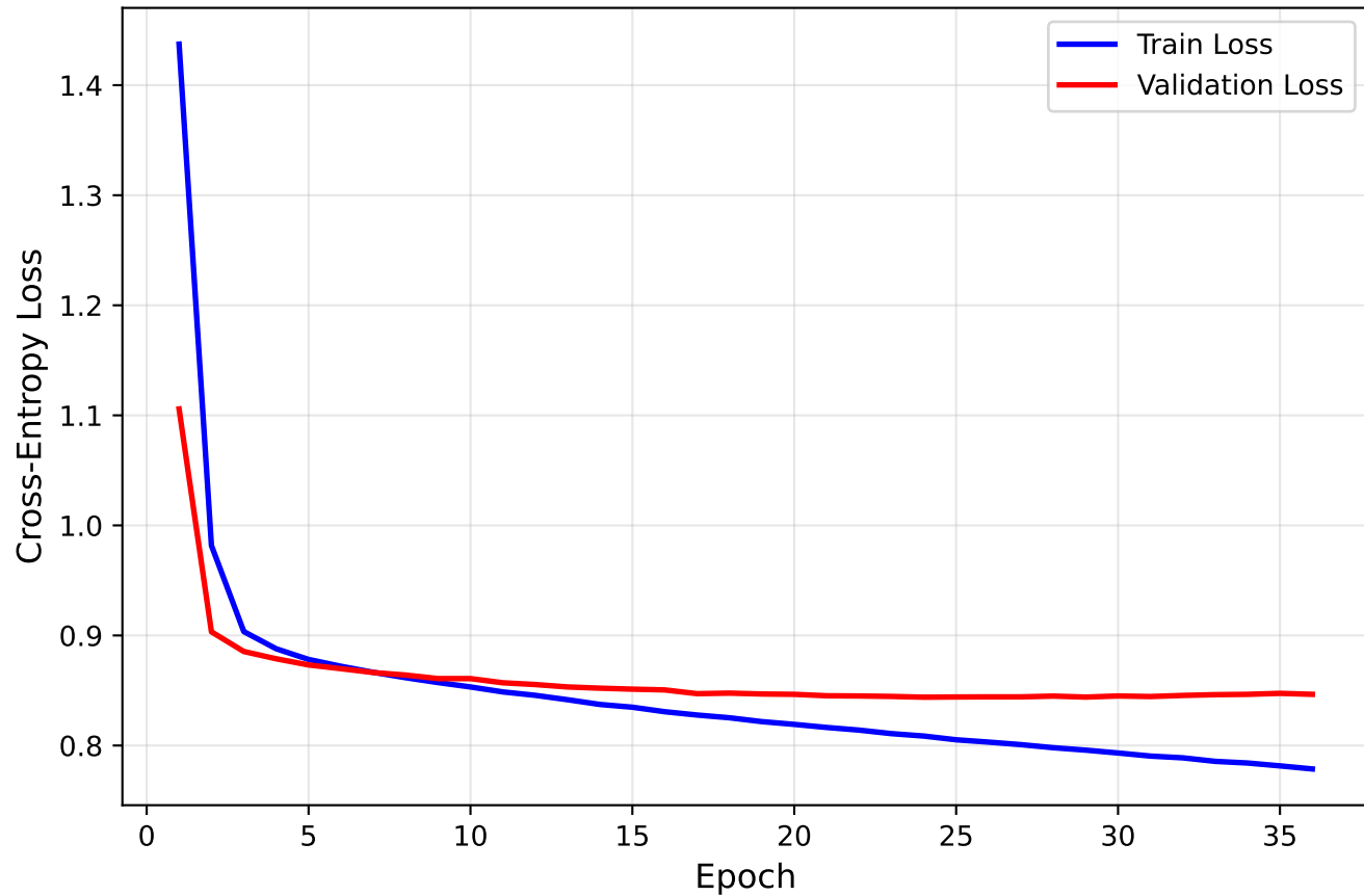
Learning Curves: Loss
