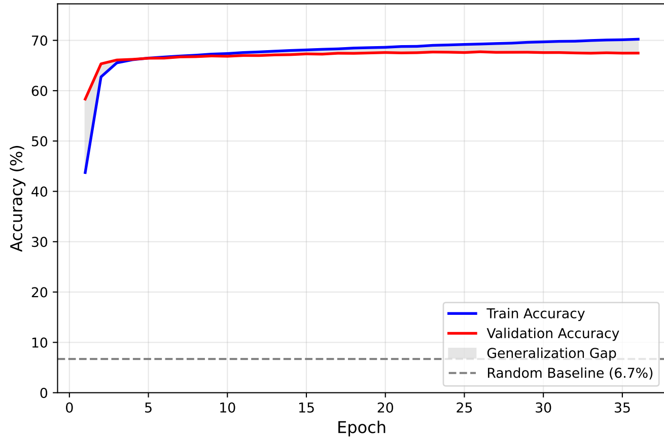
Learning Curves: Accuracy
