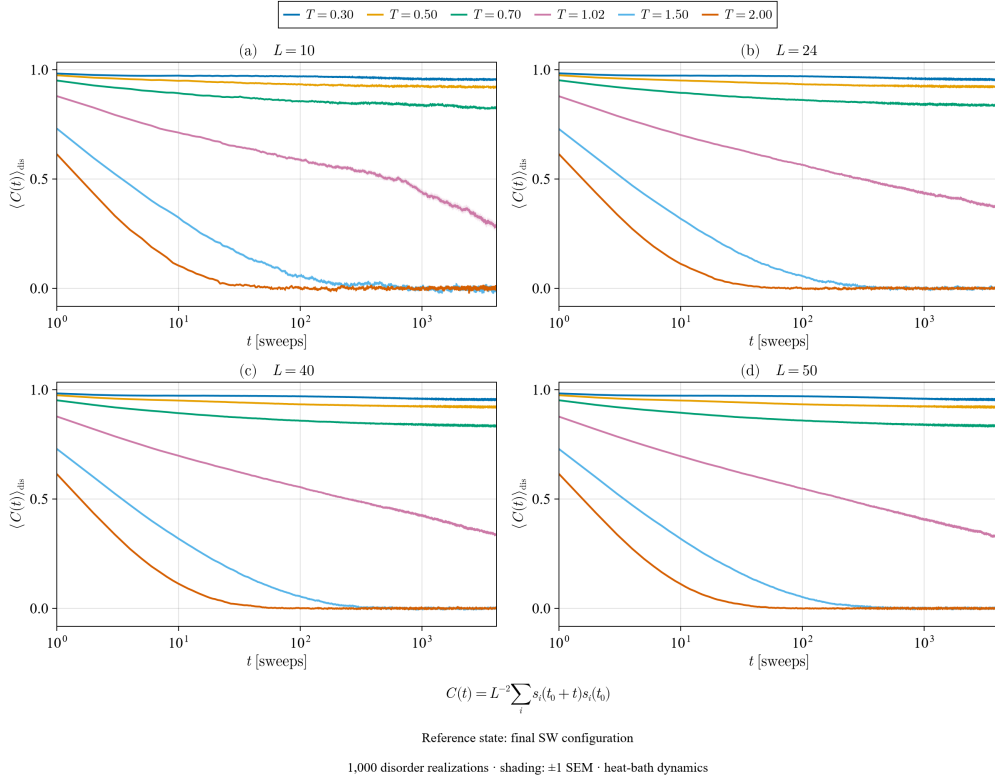
Figure 5: Disorder-averaged overlap with \pm 1 SEM. One time unit is one random-site heat-bath sweep following the last SW measurement. The horizontal axis is logarithmic and the vertical axis is linear. The stored value A(0) = 1 is omitted from the logarithmic time axis; nonpositive estimates and full SEM bands are retained.
