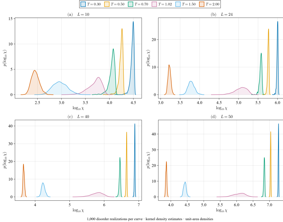
Figure 4: Distributions of total susceptibility at six temperatures for L = 10, 24, 40, 50 , normalized in d(\log_{10} \chi) . Smooth curves are kernel density estimates; narrow peaks have larger density because their areas remain unity. Small shoulders require bandwidth and sampling checks before interpretation.
