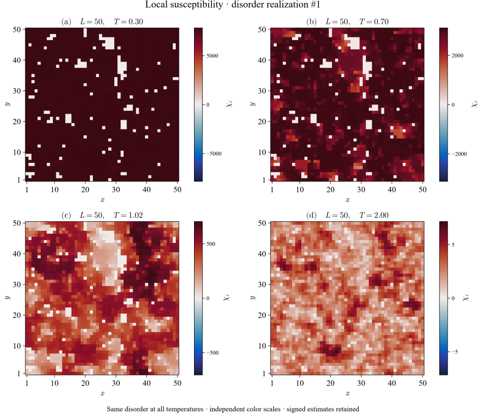
Figure 3: SW estimates of local susceptibility at T = 0.30, 0.70, 1.02, 2.00 for the same bond realization at p = 0.6 . Each panel uses an independent symmetric linear color scale. Negative estimates are retained; equal color intensity across panels does not mean equal response.
