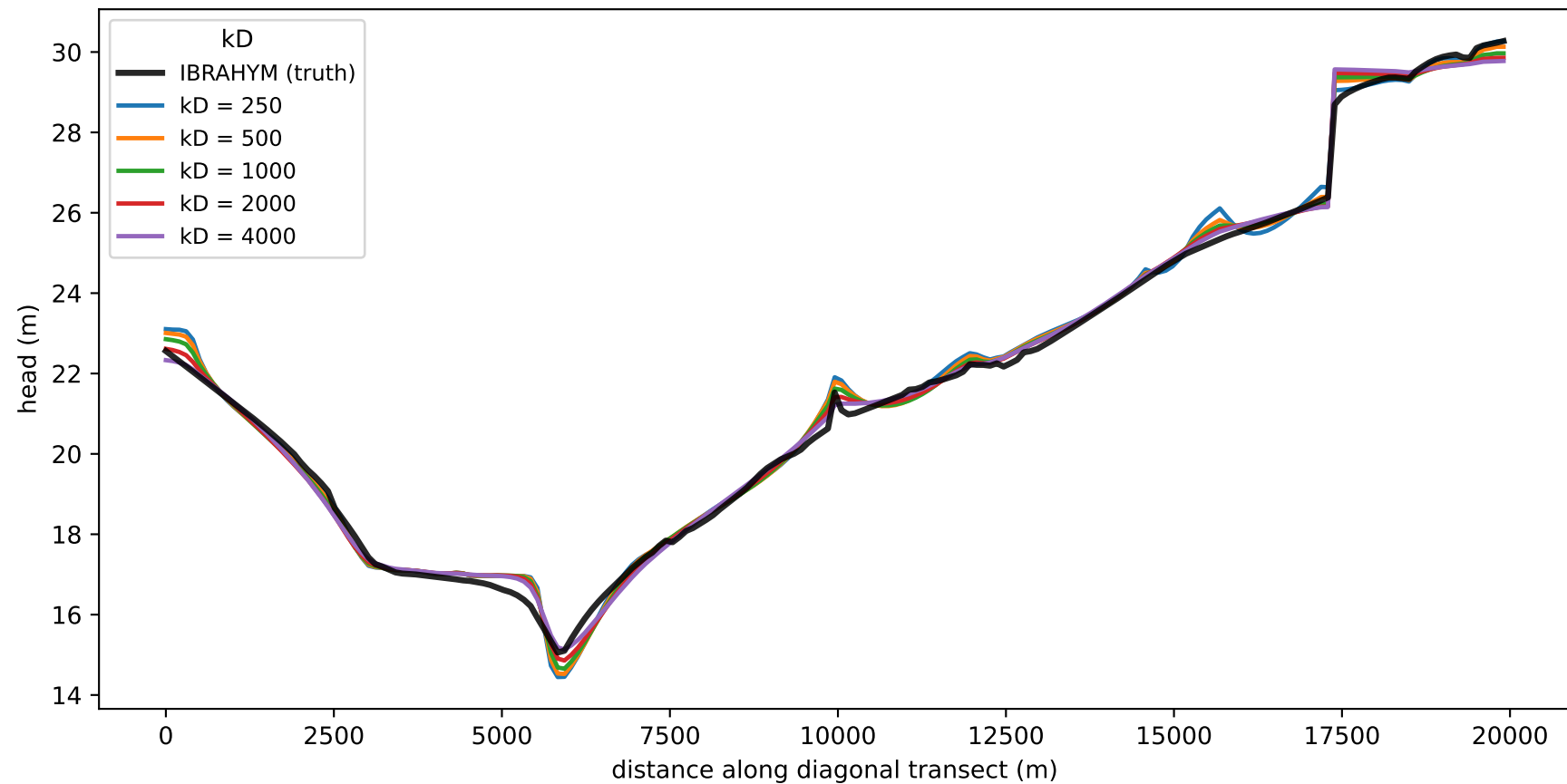
Fitted head vs. kD [ \text{m}^2/\text{day} ] (truth in black)
