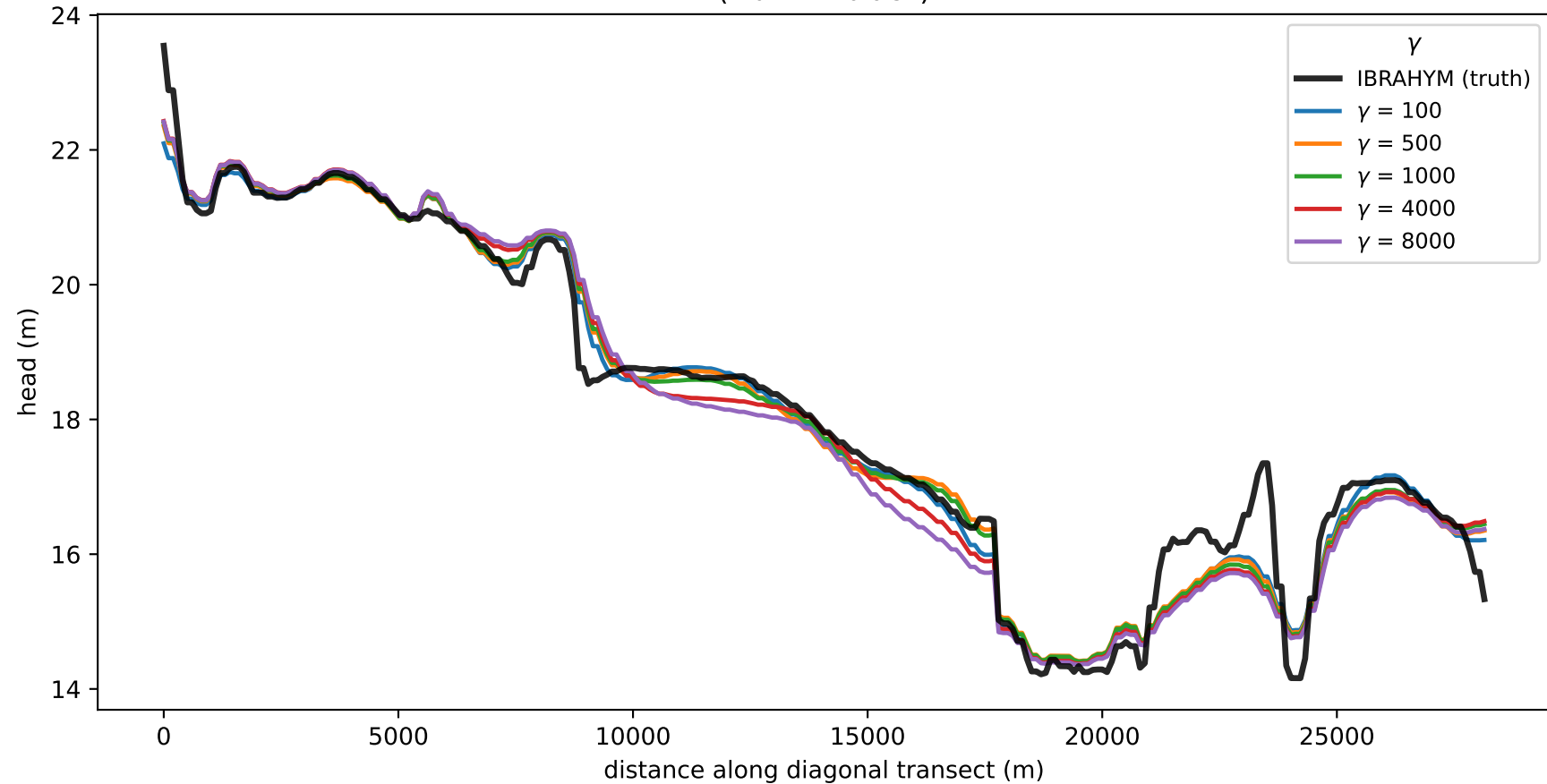
Fitted head along a diagonal transect (BL \rightarrow TR) vs. \gamma (truth in black)
