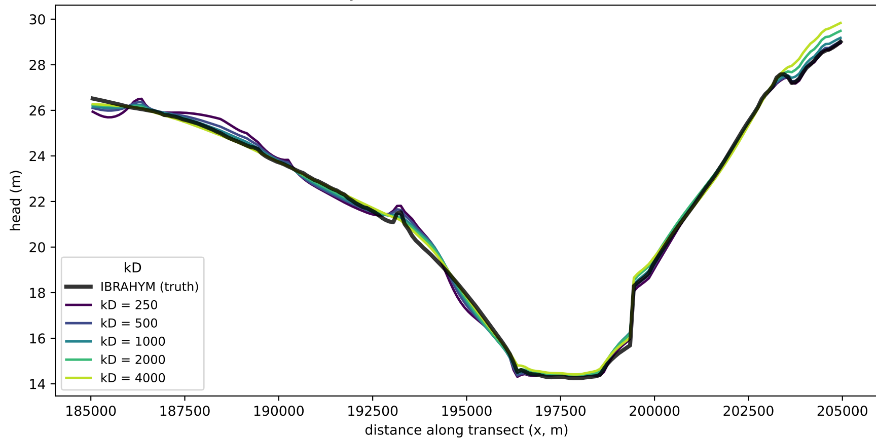
Fitted head along a mid-domain transect vs. kD [ \text{m}^2/\text{day} ] ( y = 360050 m; truth in black)
