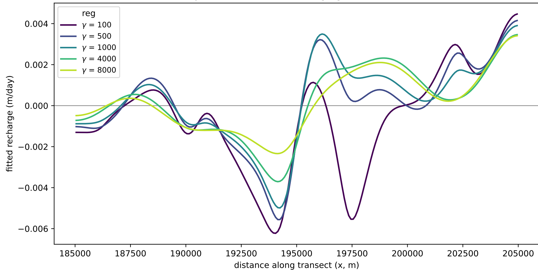
Fitted recharge along a mid-domain transect vs. \gamma ( y = 360050 m; no recharge ground truth)
