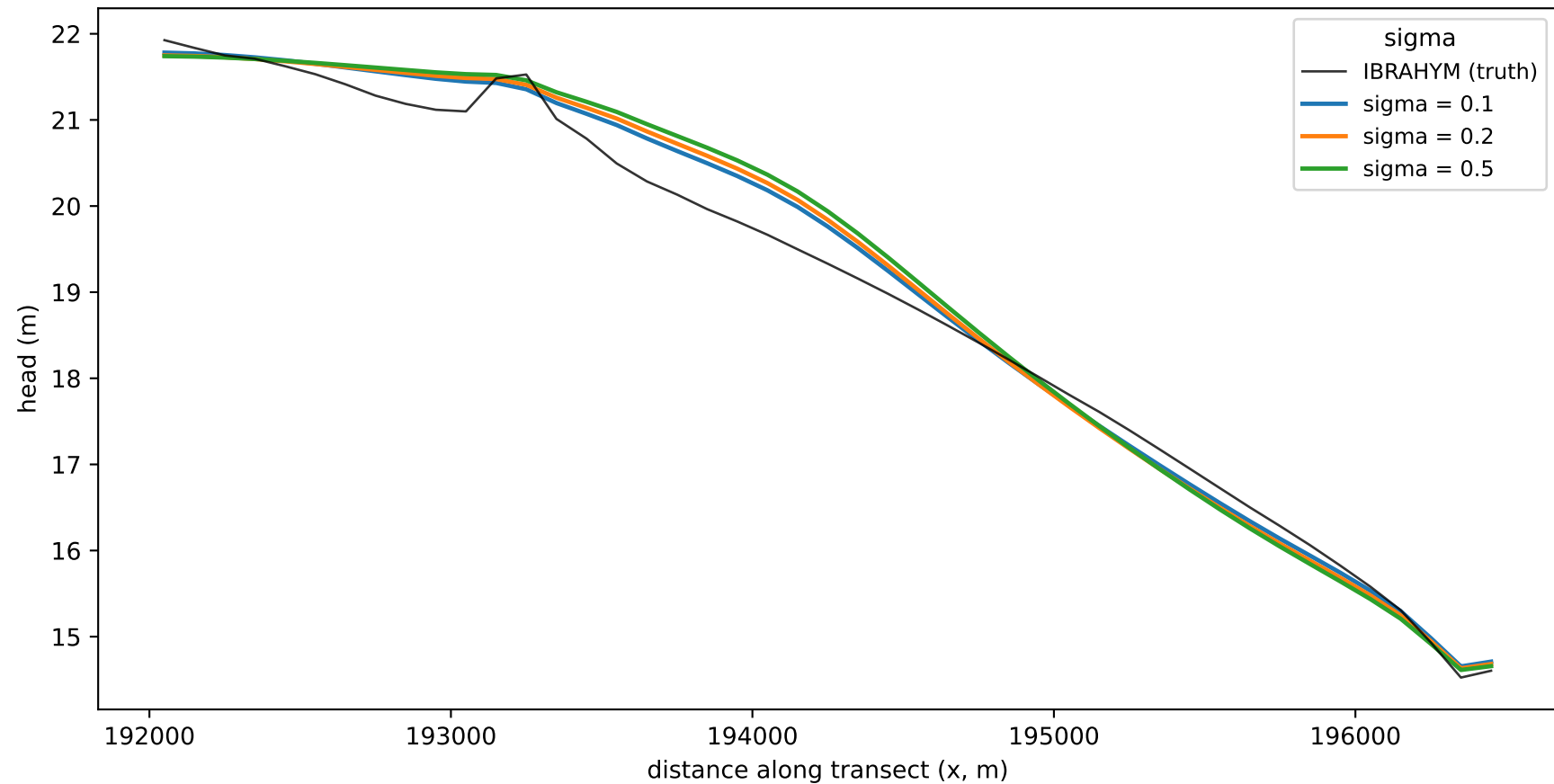
Fitted head along a mid-domain transect vs. sigma (y = 360050 m; truth in black)
