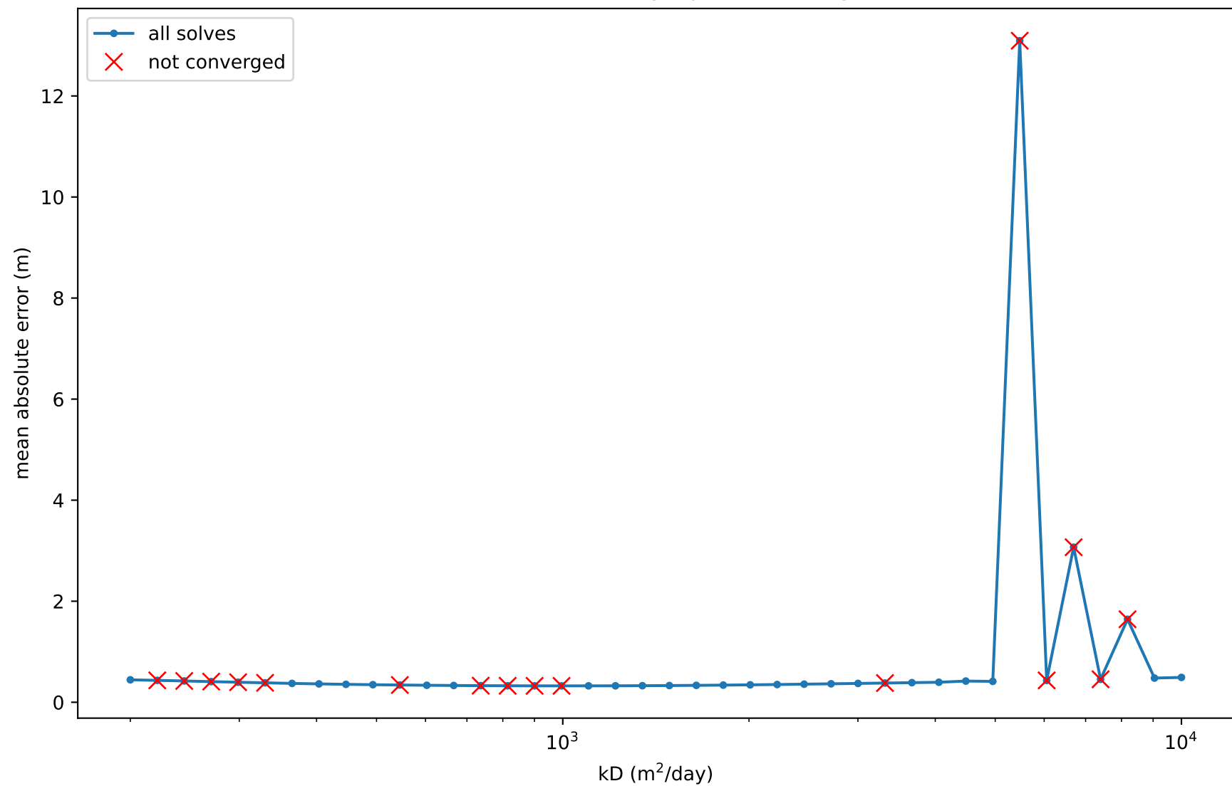
Error vs transmissivity ( \gamma = 4000 , original)
