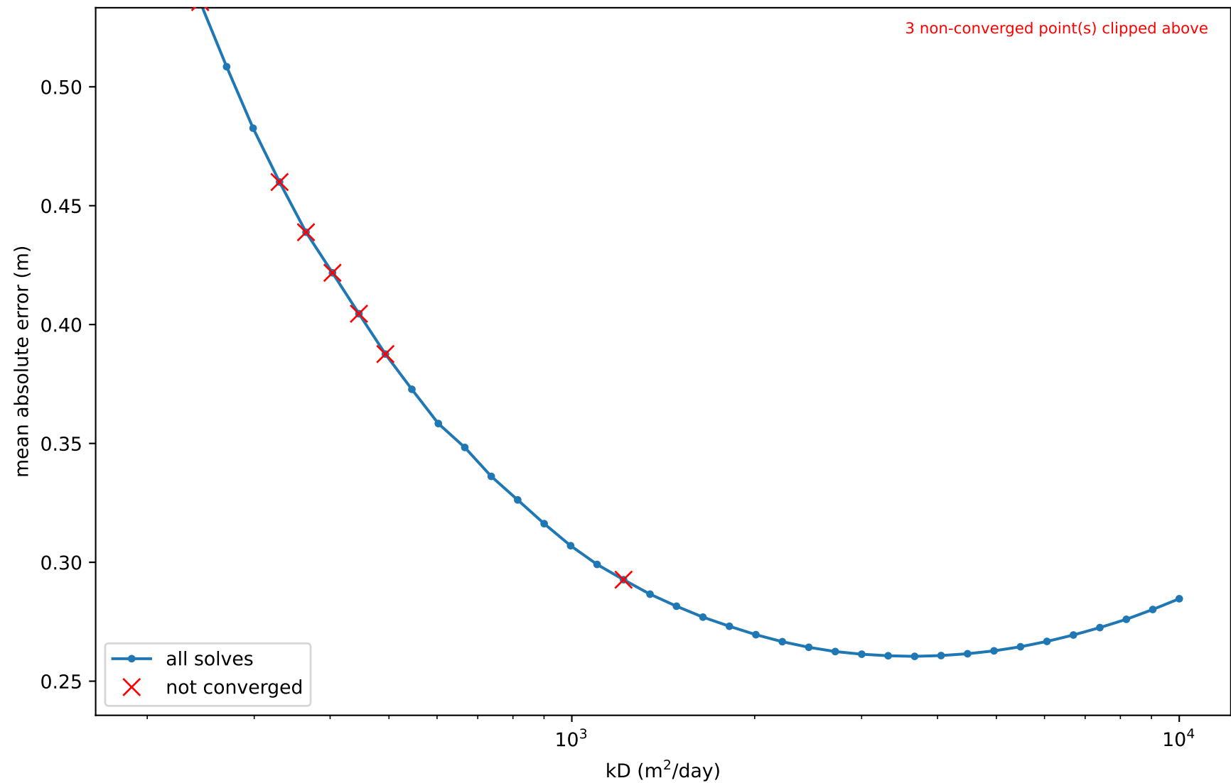
Error vs transmissivity ( \gamma = 100 , original)
