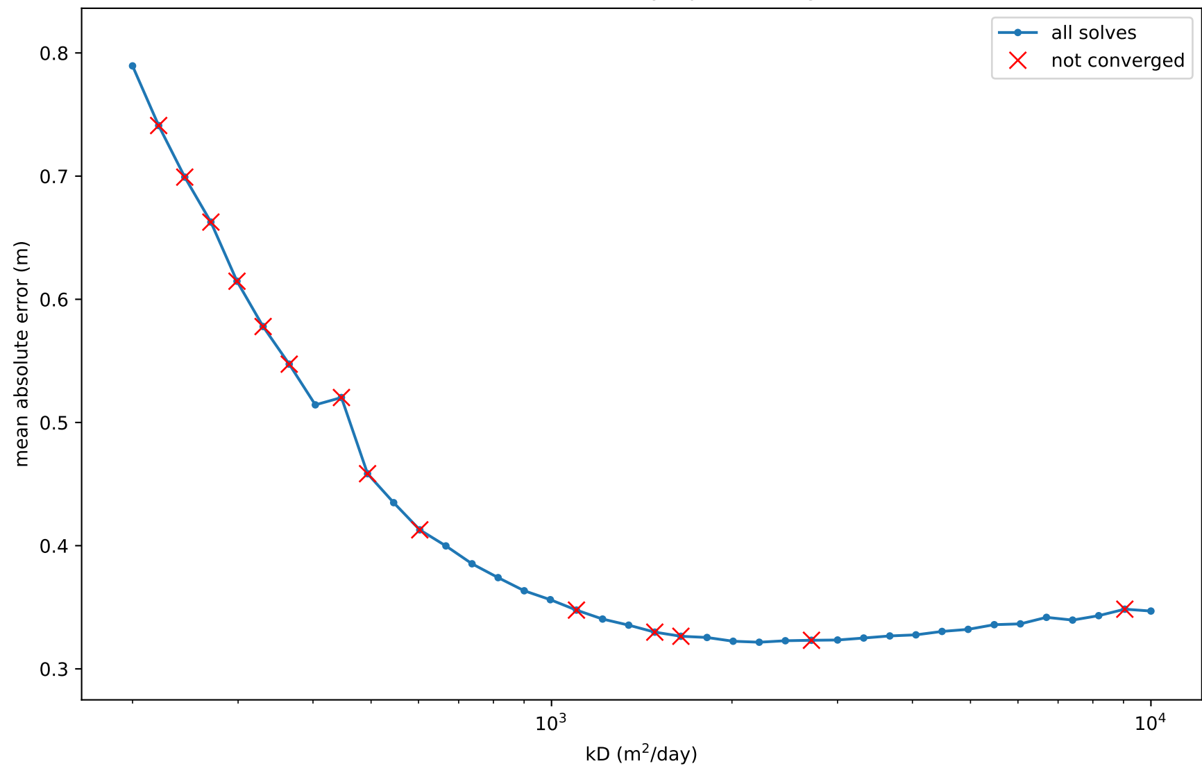
Error vs transmissivity ( \gamma = 10 , original)
