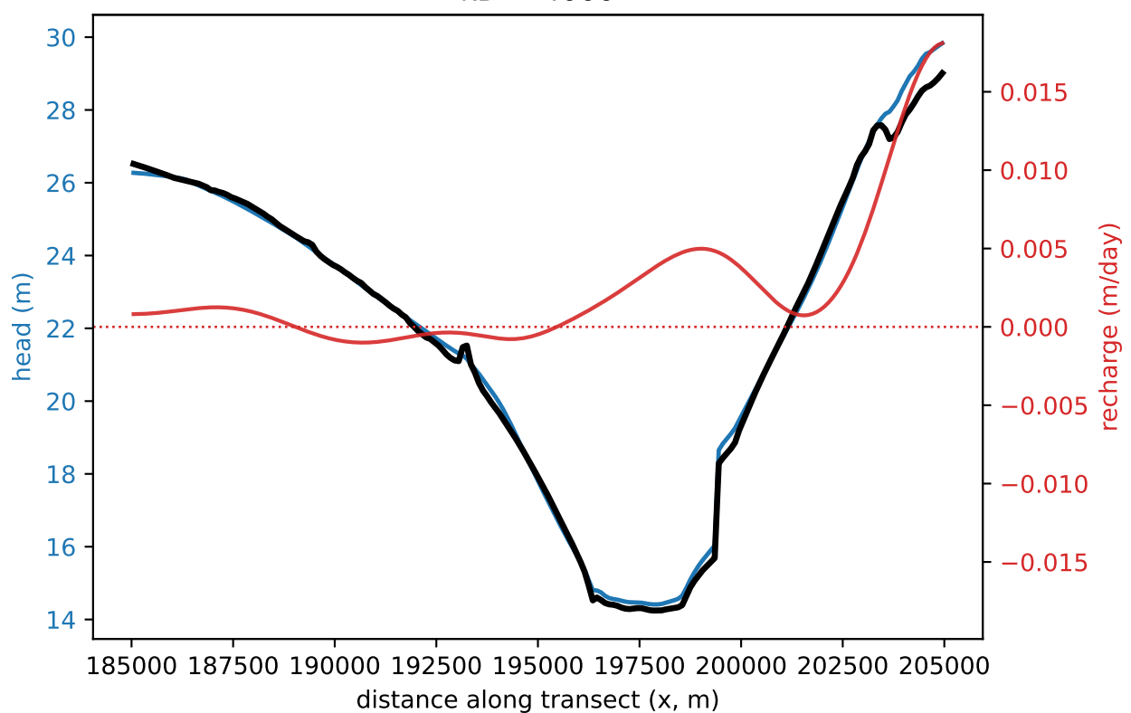
Head (blue, left) vs. recharge (red, right) along a transect ( y = 360050 m) recharge axis symmetric about zero
