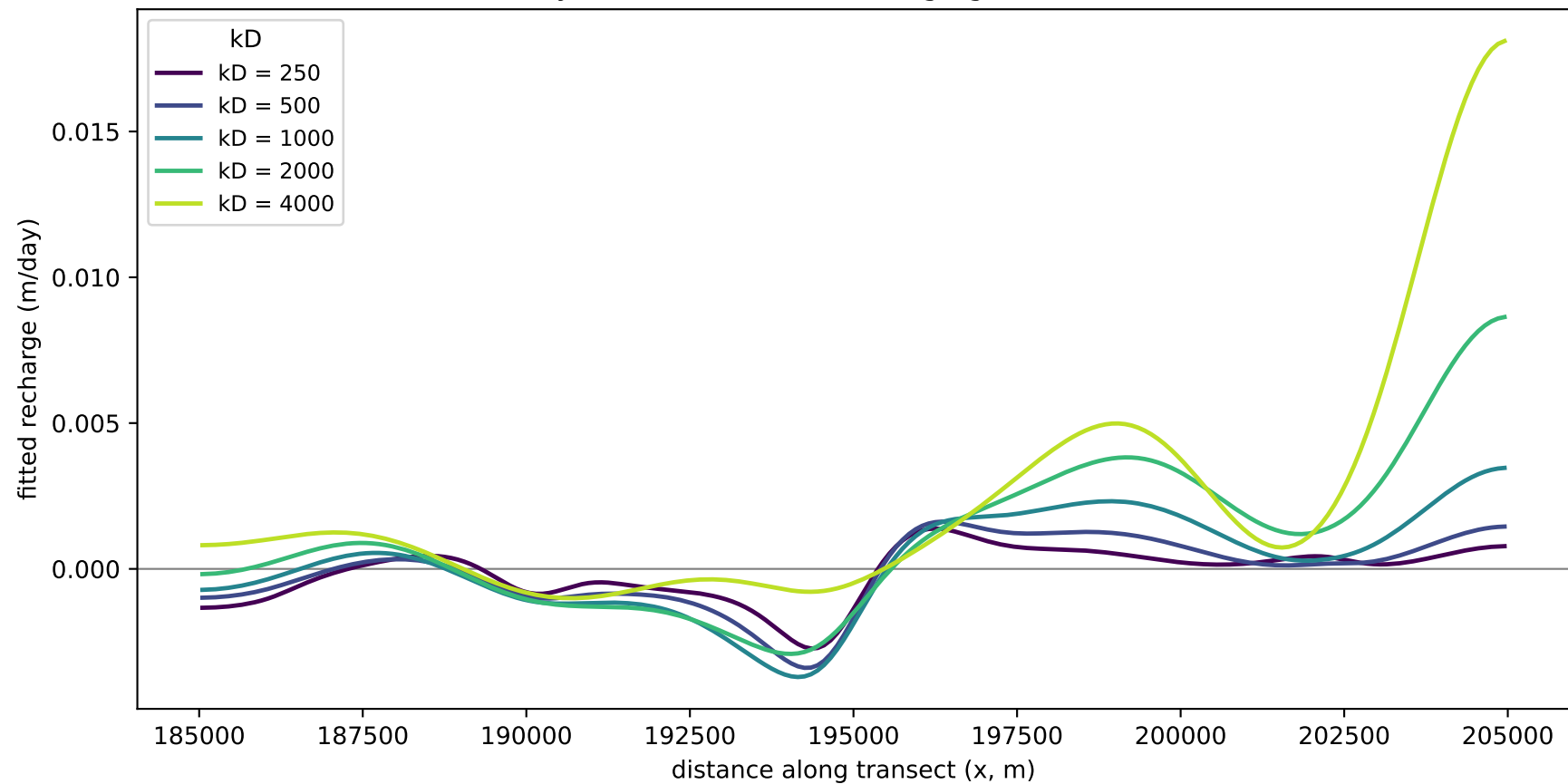
Fitted recharge along a mid-domain transect vs. kD [ \text{m}^2/\text{day} ] ( y = 360050 m; no recharge ground truth)
