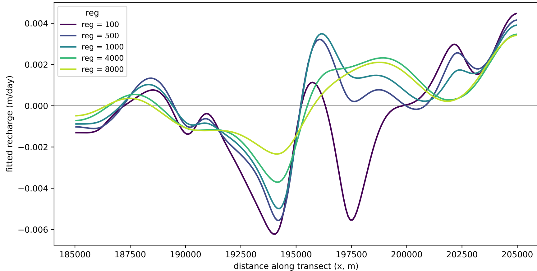
Fitted recharge along a mid-domain transect vs. reg (y = 360050 m; no recharge ground truth)
