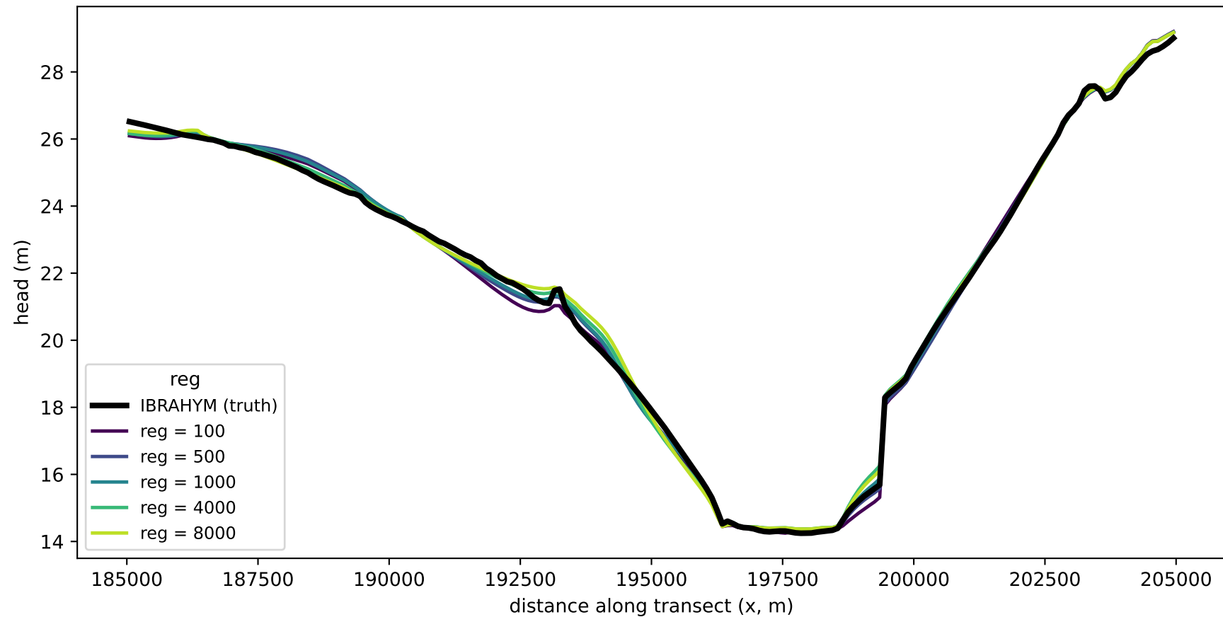
Fitted head along a mid-domain transect vs. reg (y = 360050 m; truth in black)
