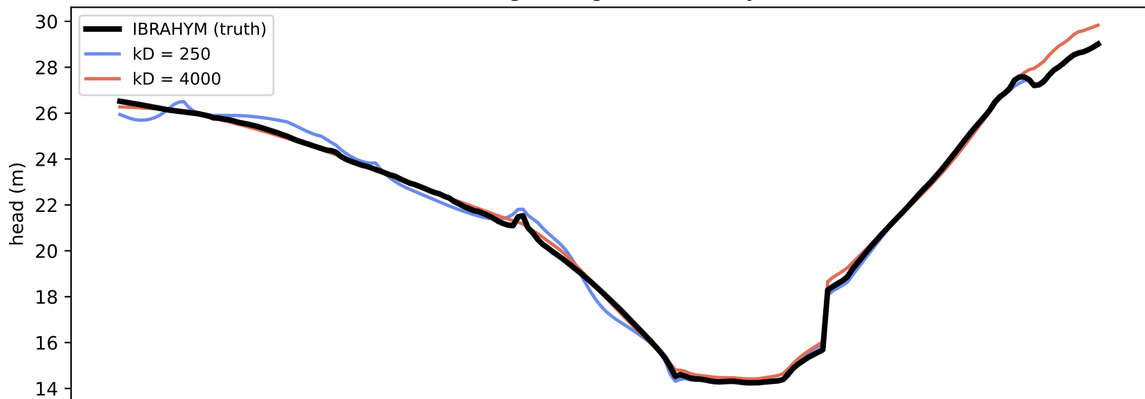
Head fit vs. recharge along a transect ( y = 360050 m)
