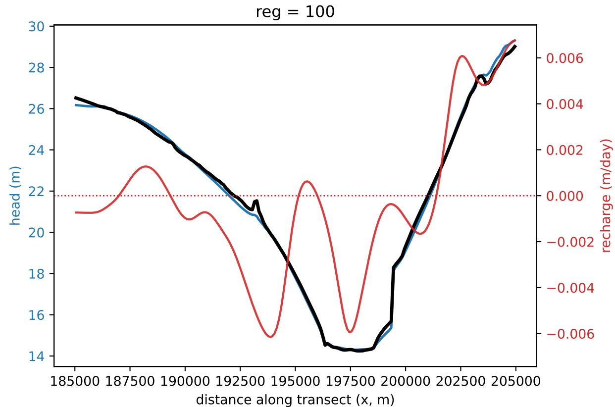
Head (blue, left) vs. recharge (red, right) along a transect ( y = 360050 m) recharge axis symmetric about zero
