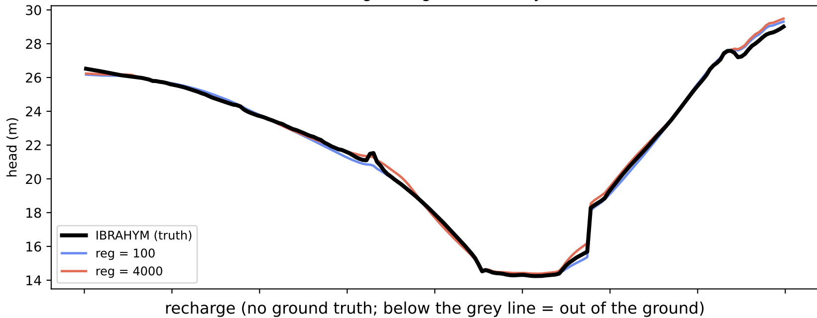
Head fit vs. recharge along a transect ( y = 360050 m)
