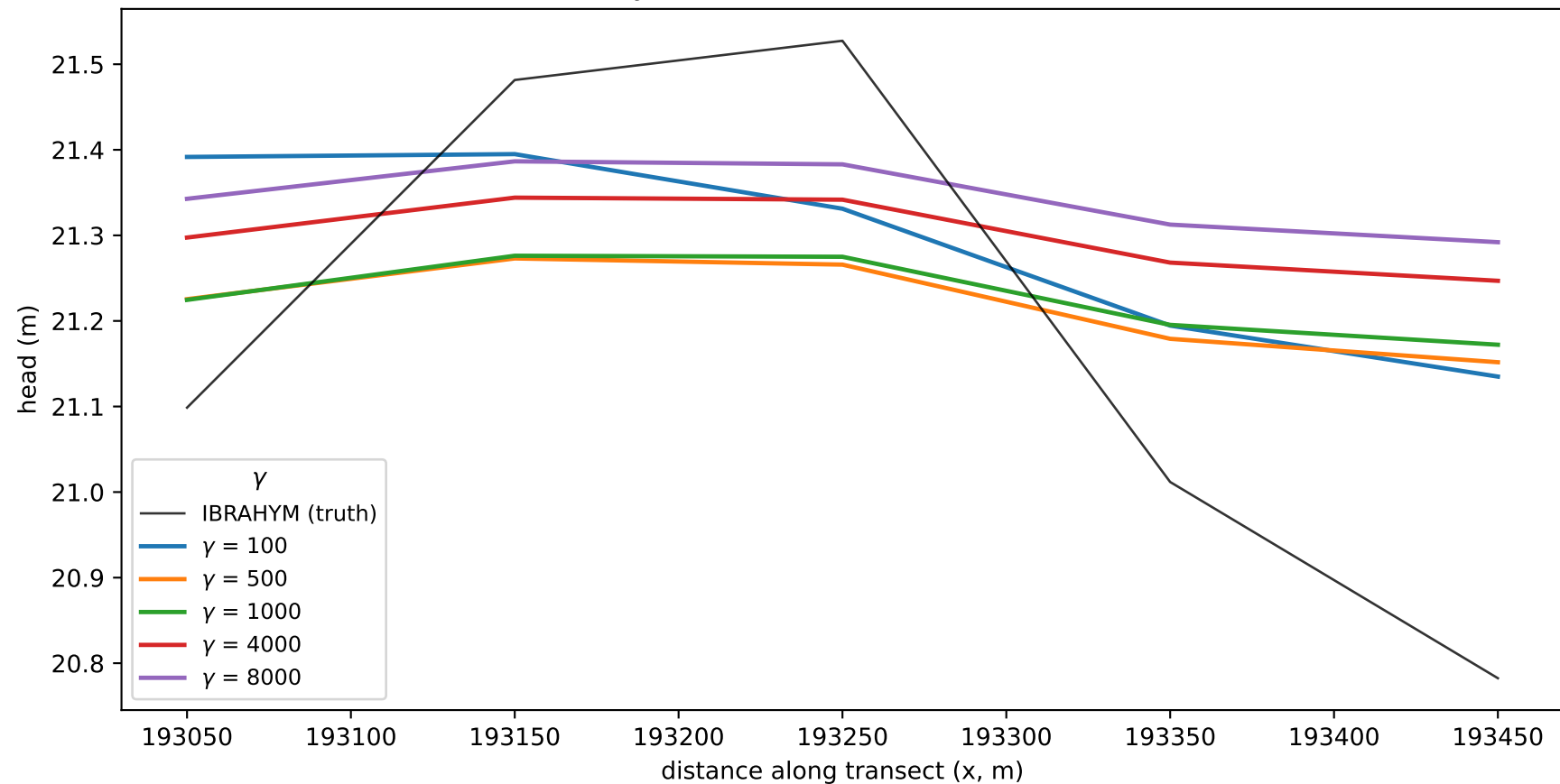
Fitted head along a mid-domain transect vs. \gamma ( y = 360050 m; truth in black)
