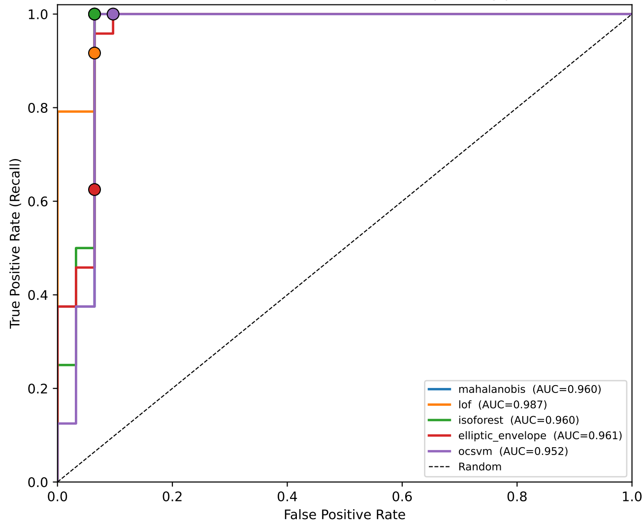
ROC Curves (dots = LOO threshold operating point)
