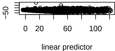
Resids vs. linear pred.
