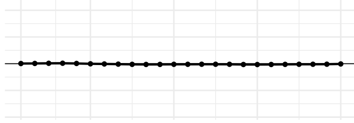
SR
