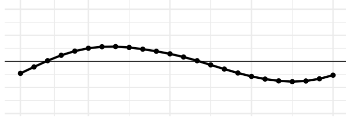
WS
