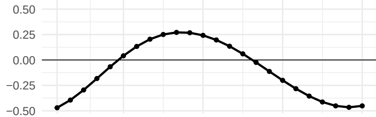
TEMP
