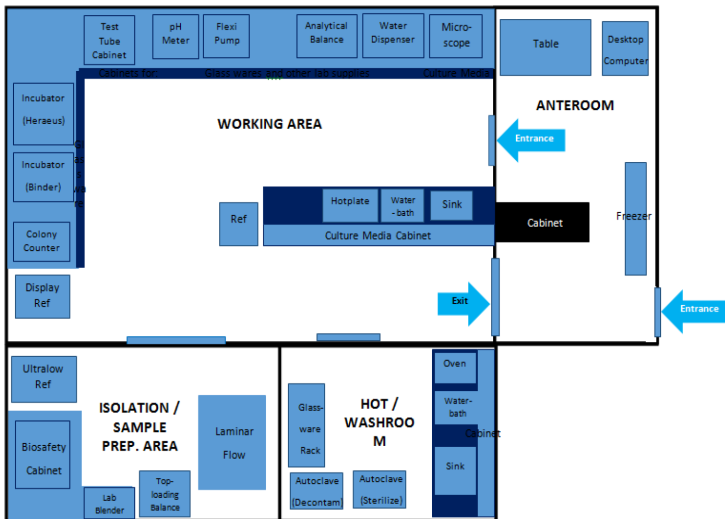
Microbiology Laboratory Instrumental Layout
