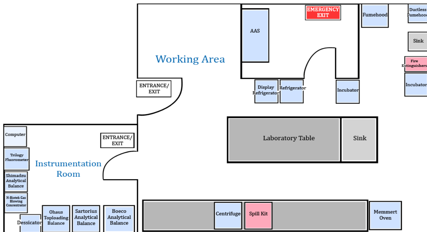
Chemistry Laboratory Instrumental Layout
