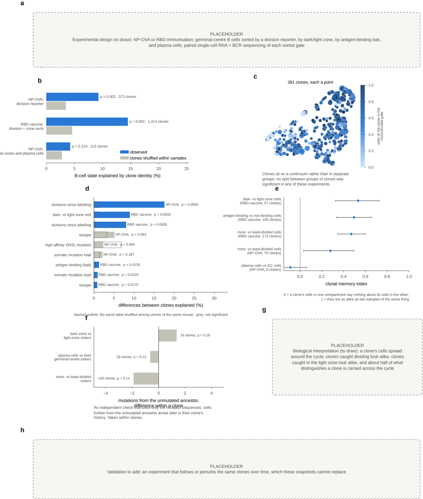
Figure 2 | Germinal-centre clones differ along a continuum of selection
