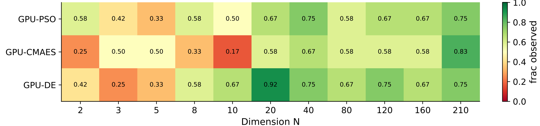
Fraction of budget cells taken from real history (1=all observed)
