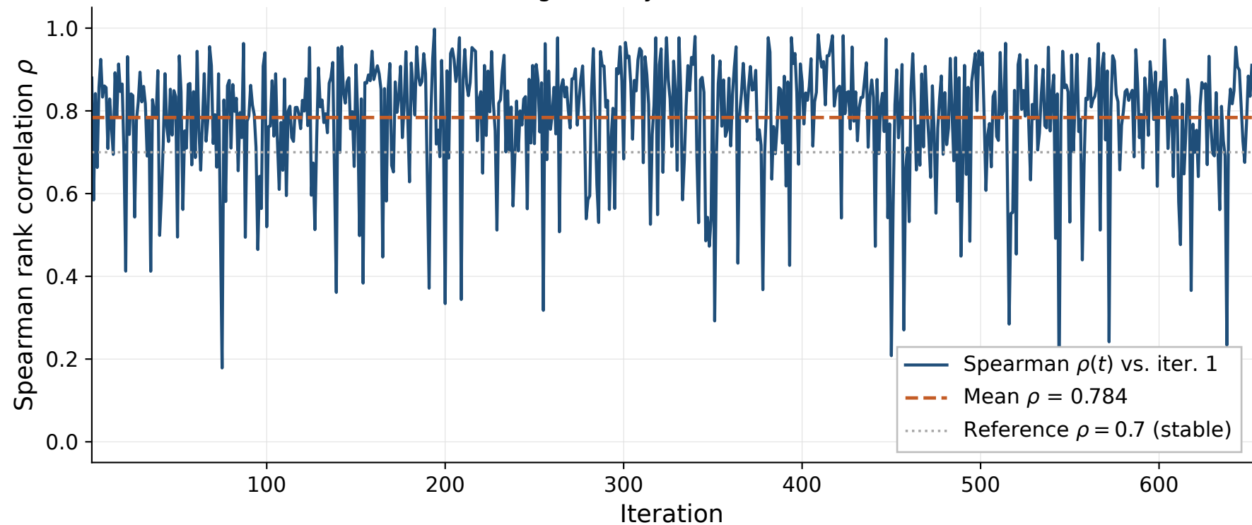
Ranking stability over GD iterations
