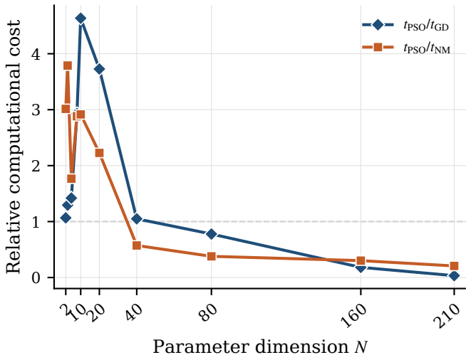
(f) Relative cost of PSO
