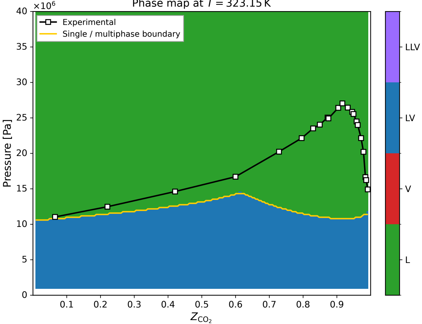
Phase map at T = 323.15 K
