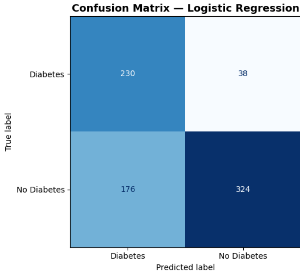
Figure 4: Final Model- Confusion matrix
